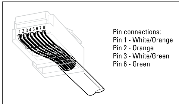
Figure 3-1: Attaching an RJ-45 connector to twisted- pair cable.
