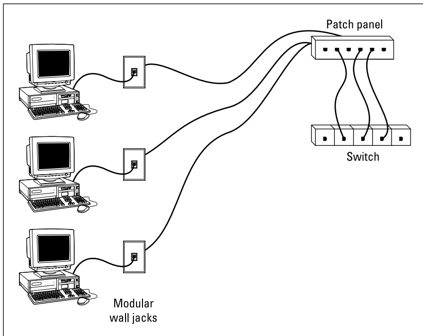
Figure 3-2: Using wall jacks and patch panels.
